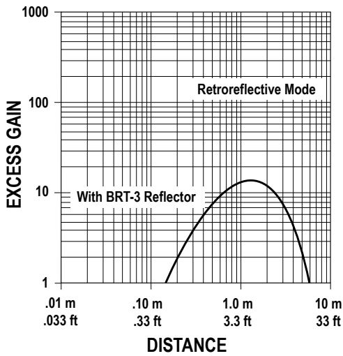
Figure 3. Excess Gain
