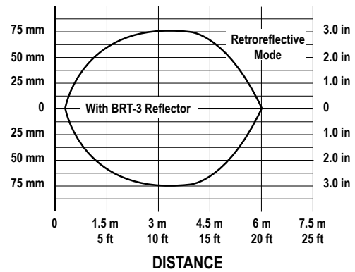
Figure 4. Beam Pattern
