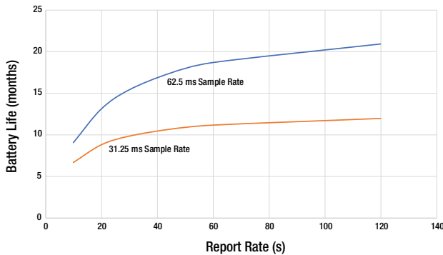
Battery Life for 900 MHz Radios
