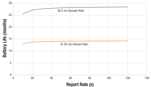
Battery Life for 2.4 GHz Radios
